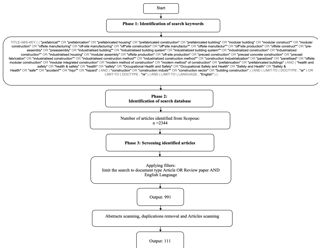
Figure 1: PRISMA Flowchart
